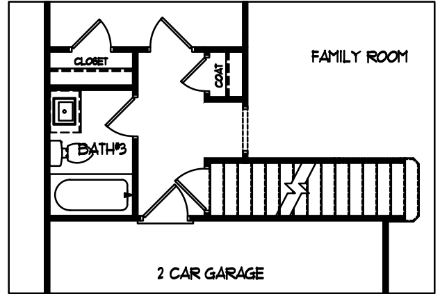
STAIRS ON BASEMENT CONDITION
