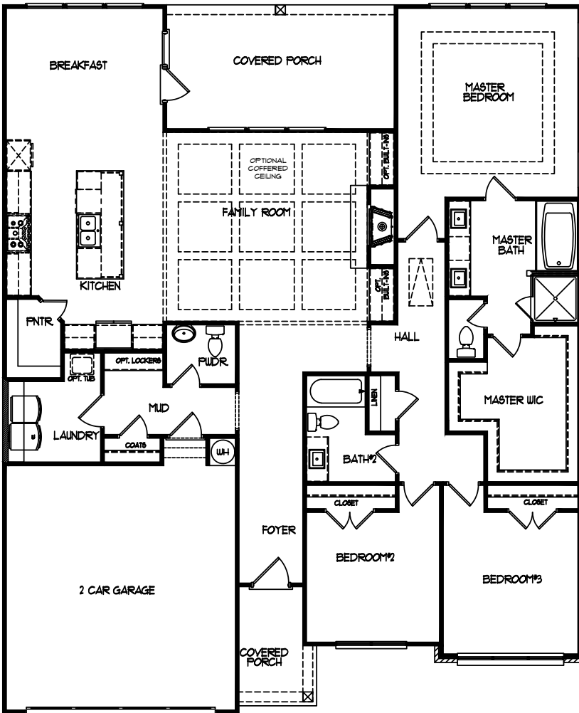
FIRST FLOOR
