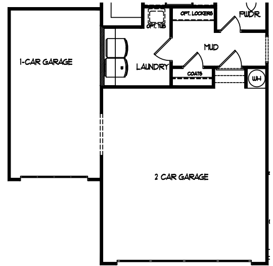
OPT. 3RD CAR GARAGE
