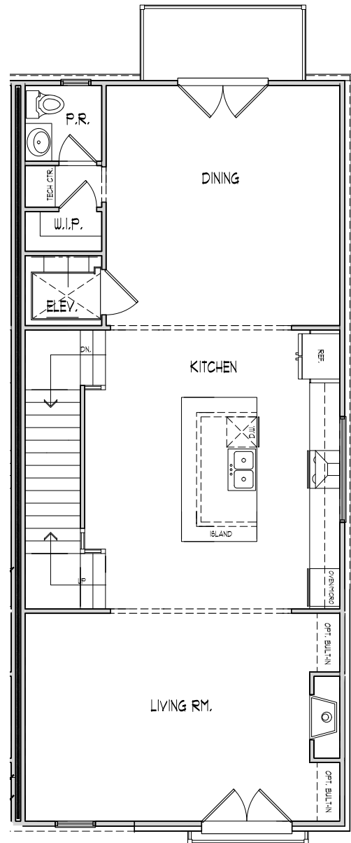
SECOND FLOOR
