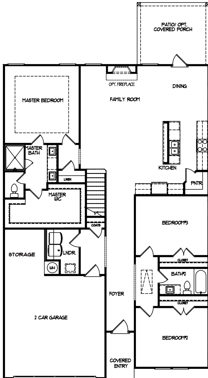
MAIN FLOOR
