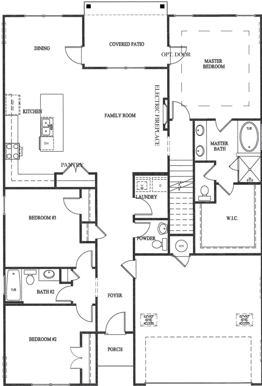
FIRST FLOOR
