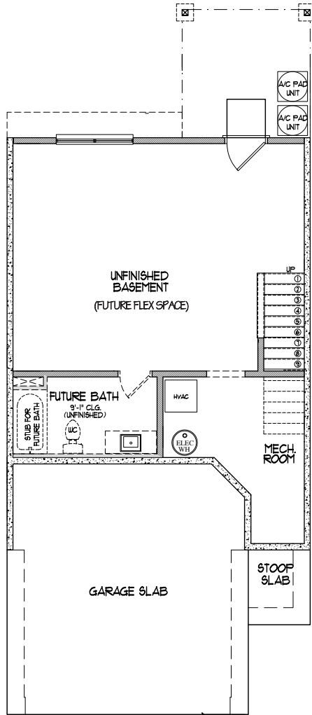
BASEMENT LEVEL W/ FUTURE FLEX SPACE
