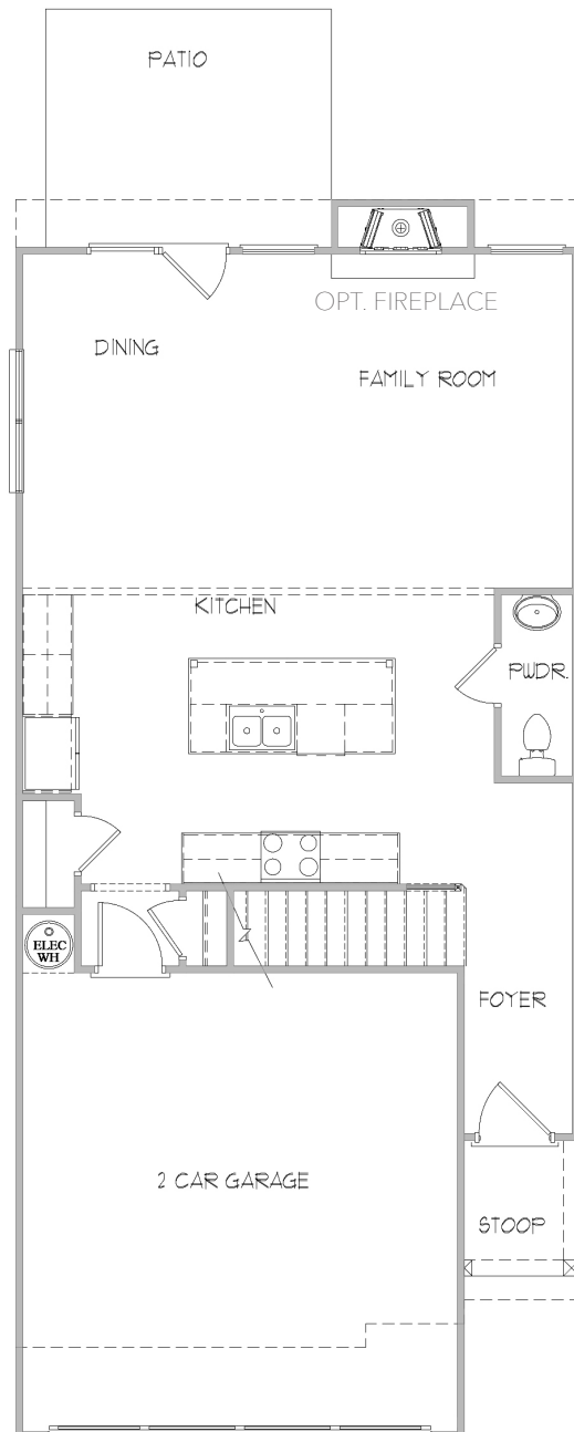
MAIN LEVEL
