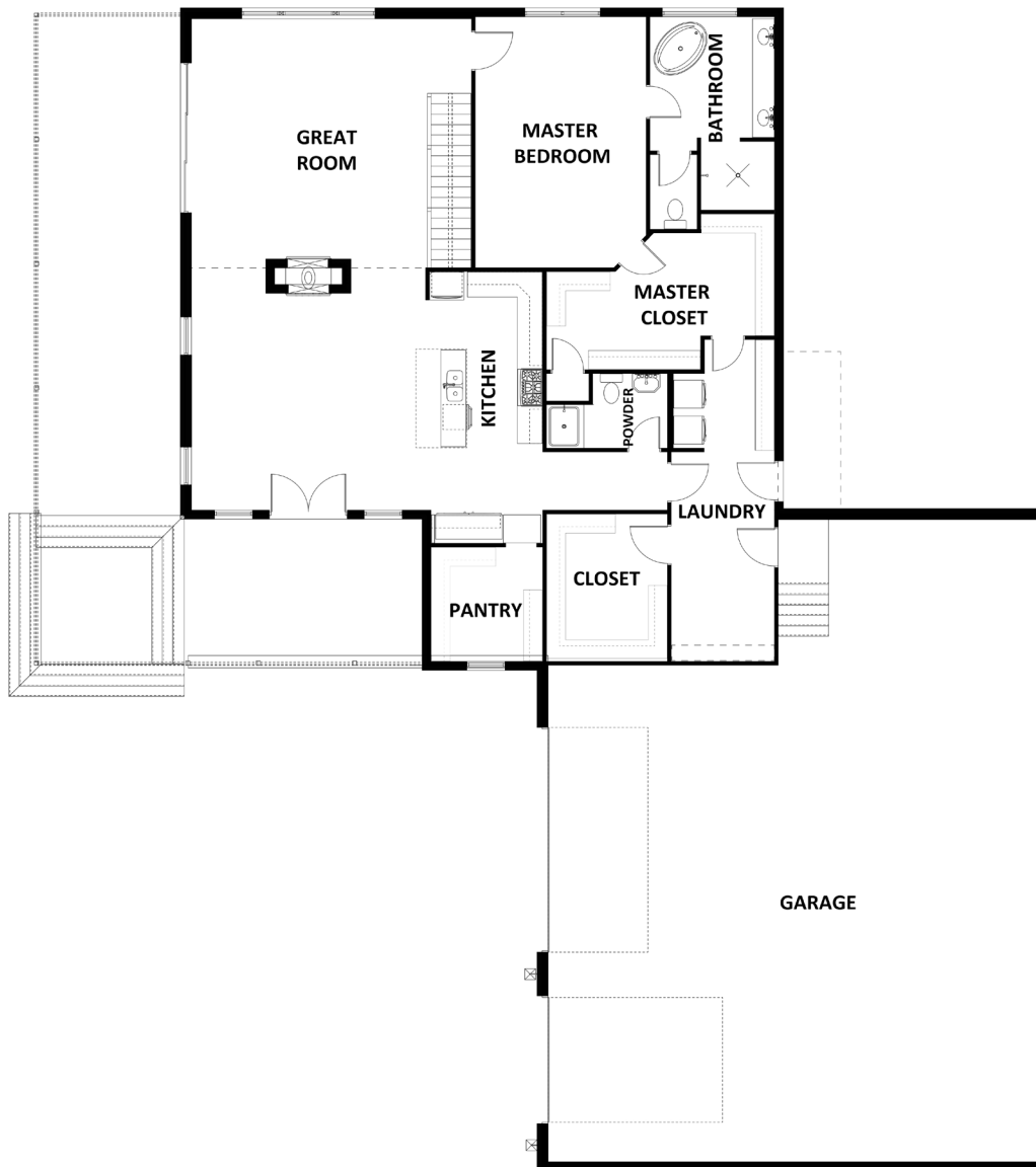
MAIN FLOOR
