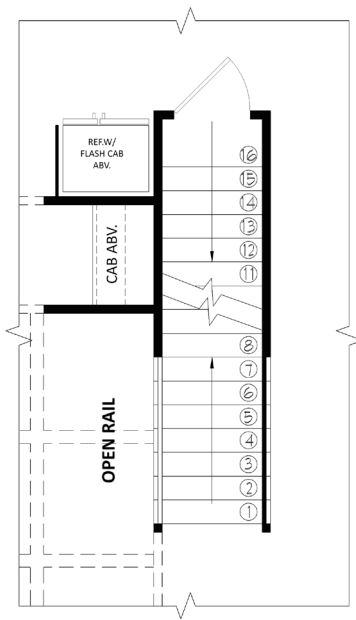
First Floor Plan w/ Opt. Basement
