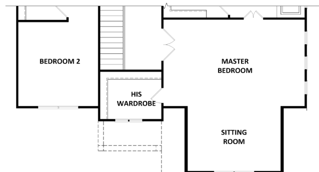
Second Floor Plan w/ Opt. 2nd Closet
