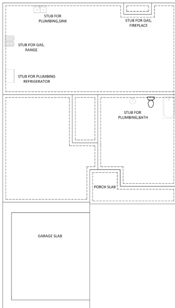
SLAB FLOOR PLAN
