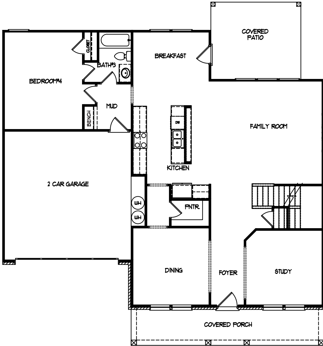
MAIN FLOOR
