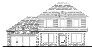
ELEVATION C
