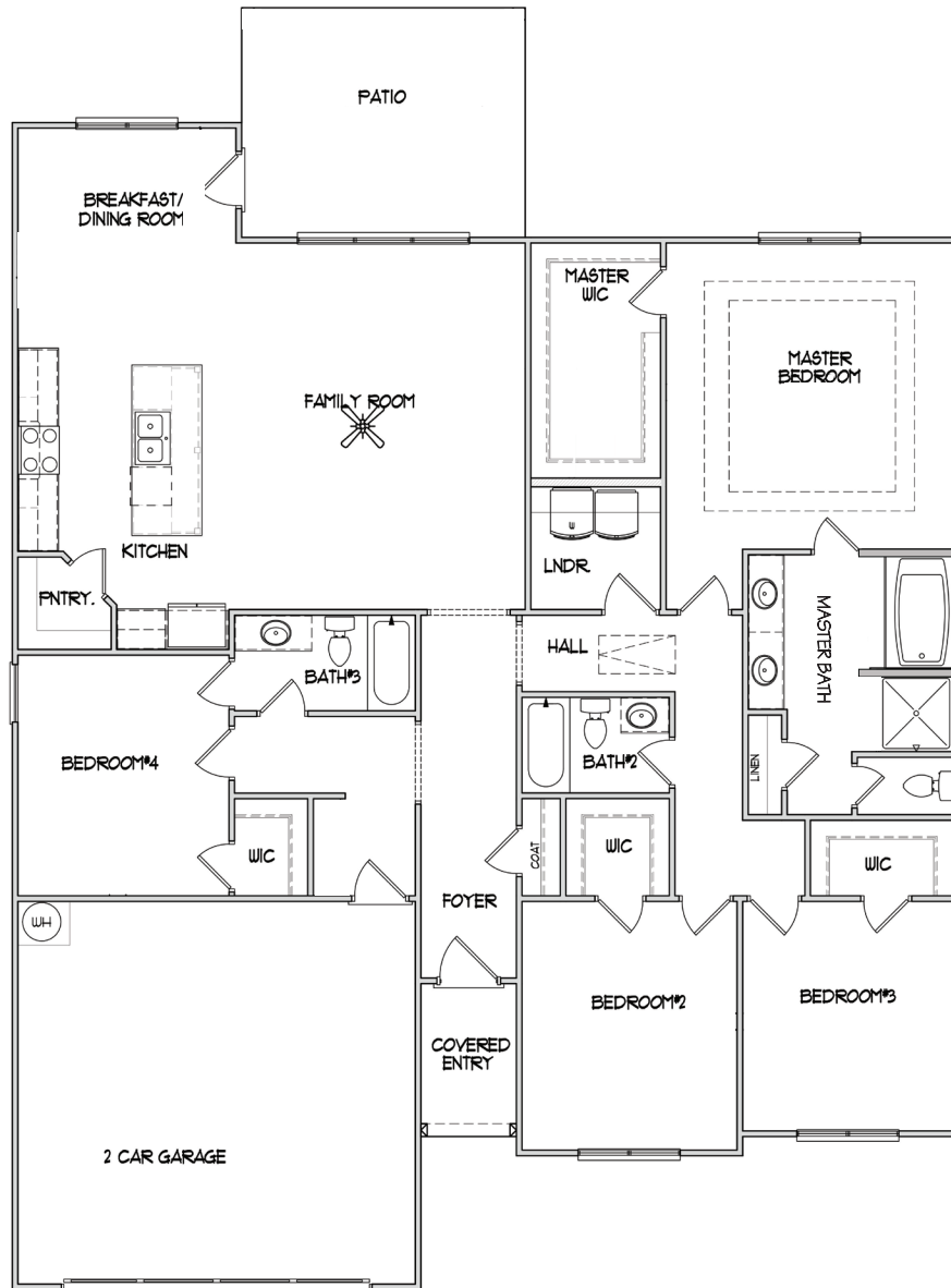
MAIN FLOOR
