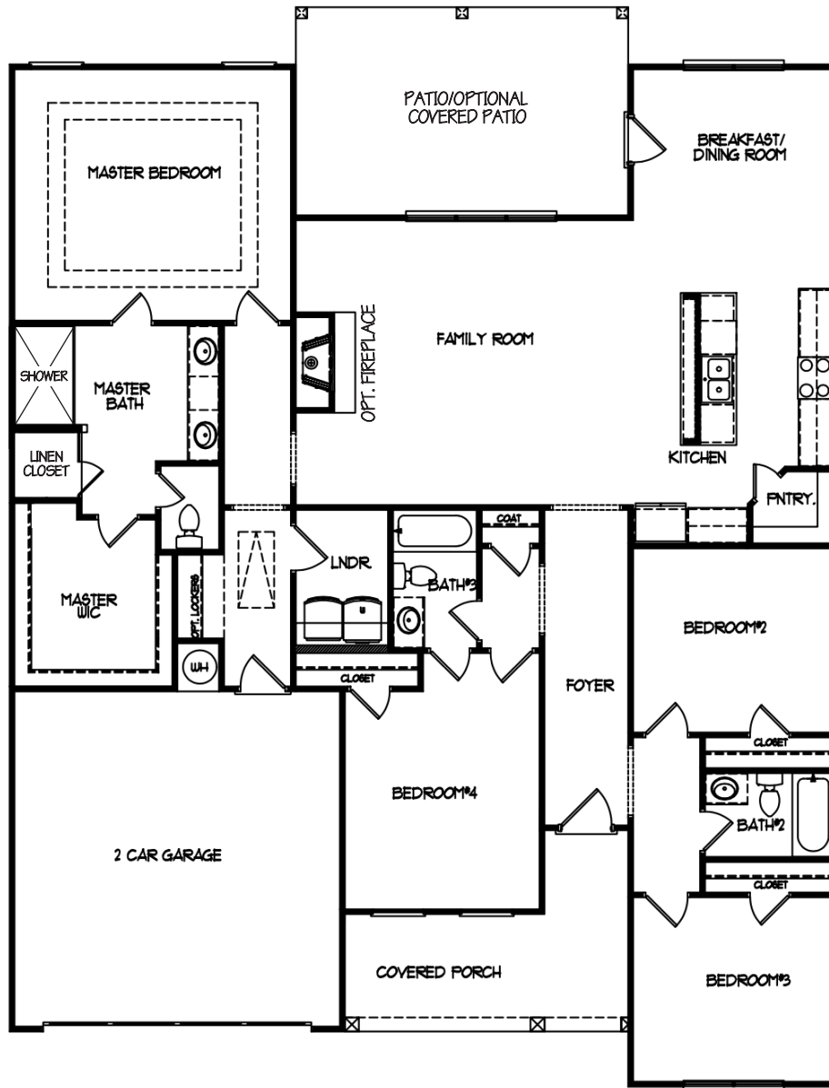
MAIN FLOOR
