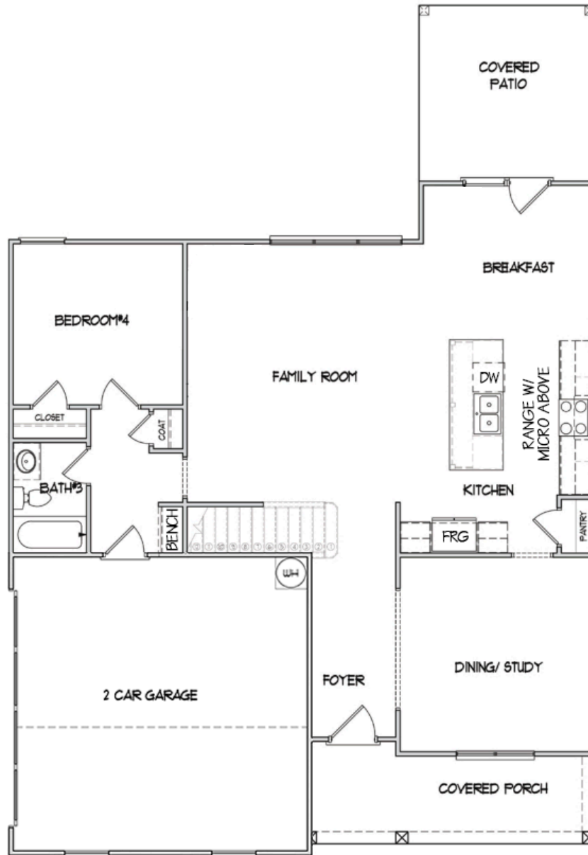
MAIN FLOOR
