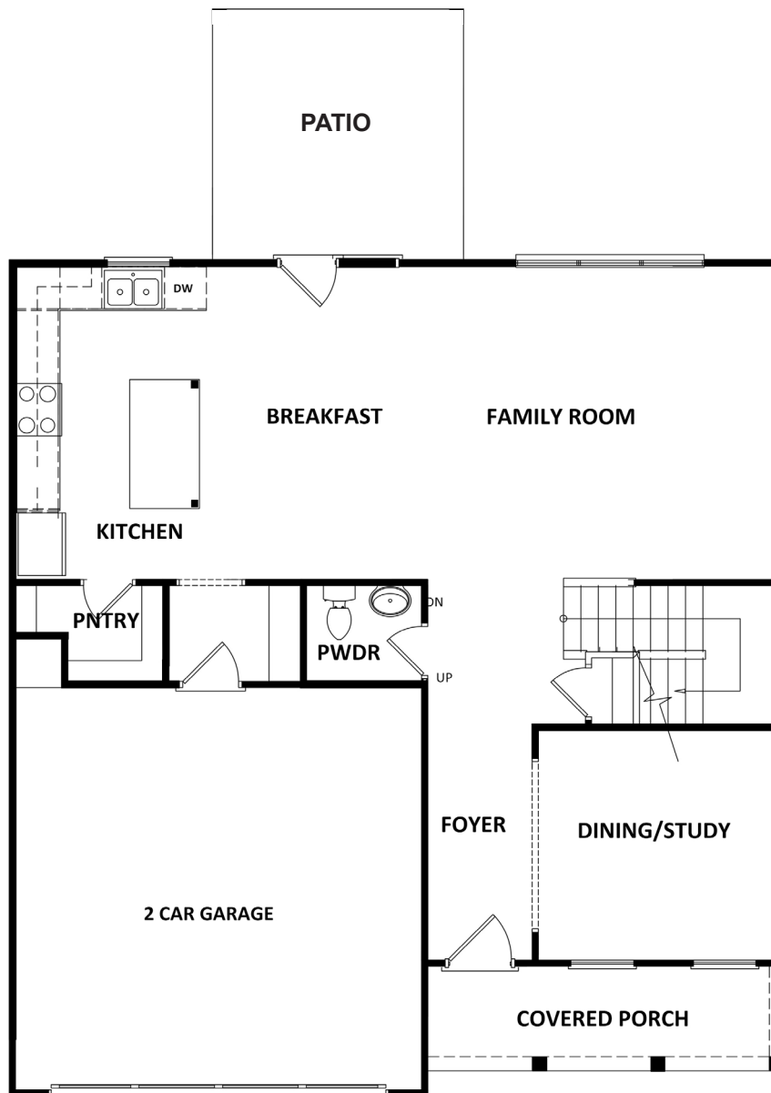
MAIN FLOOR
