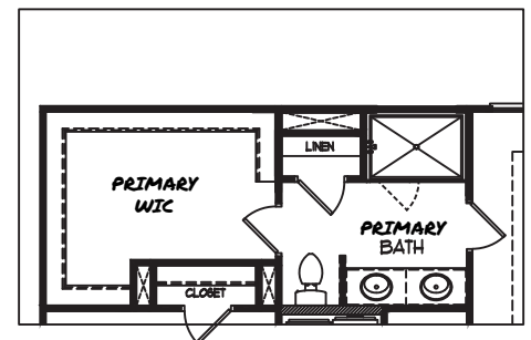
OPT. PRIMARY BATH SUPER SHOWER (PRE-SALE ONLY)
